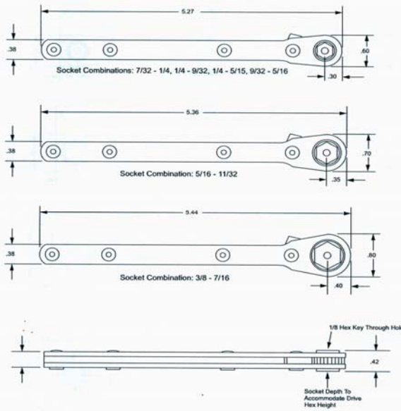
Ratchets supplied with plastic handle grip sleeve
